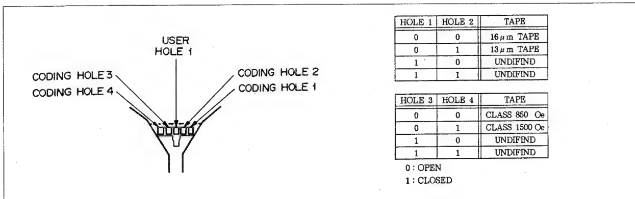
Fig. 1-2-2. Coding Holes
